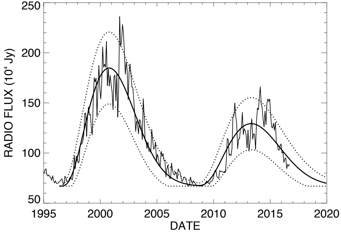
10.7cm Radio Flux Prediction (2016/10)
