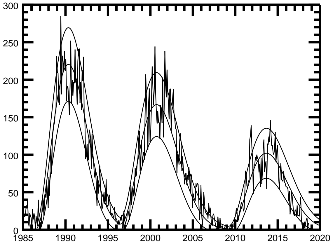
Cycle 24 Sunspot Number (V2.0) Prediction (2018/9)
